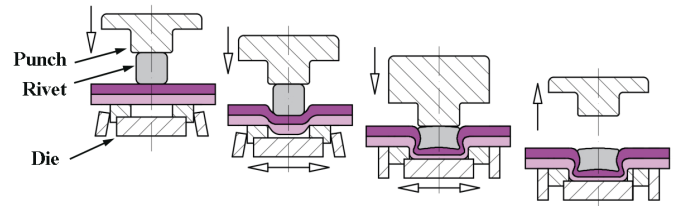
Fig. 4 Principle of clinch-ri-ving
