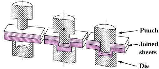
Fig. 3 Principle of clinching
