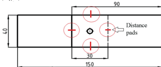
Fig. 1 Sample for the experiments (hybrid joints)
