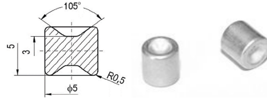
Fig. 2 Rivets for the clinch-ri-ving method
